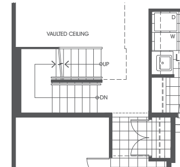
GROUND FLOOR PLAN STAIRS TO LOFT
