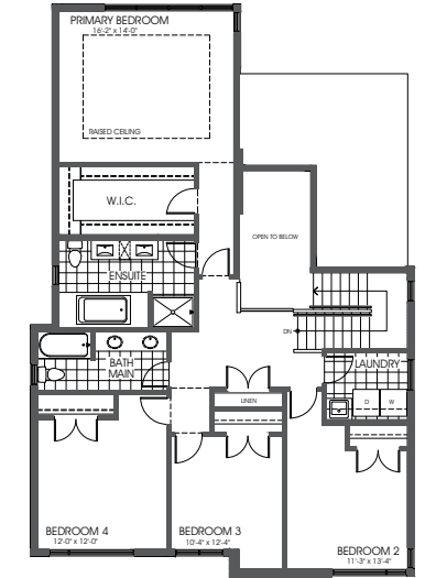
SECOND FLOOR PLAN 4-BEDROOM
