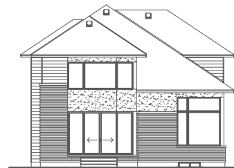
REAR ELEVATION
