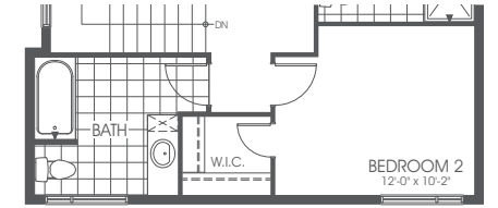
SECOND FLOOR PLAN ALTERNATE
