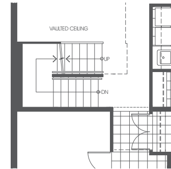
GROUND FLOOR PLAN STAIRS TO LOFT
