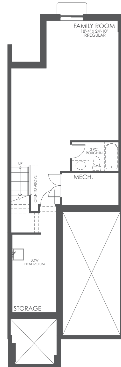
LOWER LEVEL PLAN
