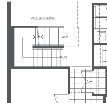
GROUND FLOOR PLAN STAIRS TO LOFT
